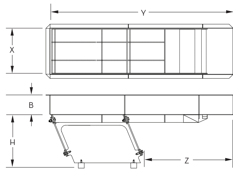
Straight Discharge
