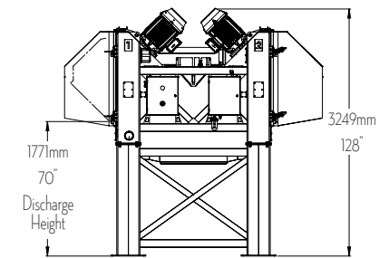
Two-drum Dryer Weight = 2730 kg (6000 lbs)
