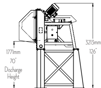
One-drum Dryer Weight = 1450 kg (3200 lbs)
