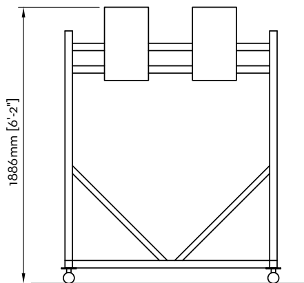
Two AVSealers on a floor stand
